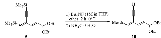
Scheme 6. Desilylation of 5
